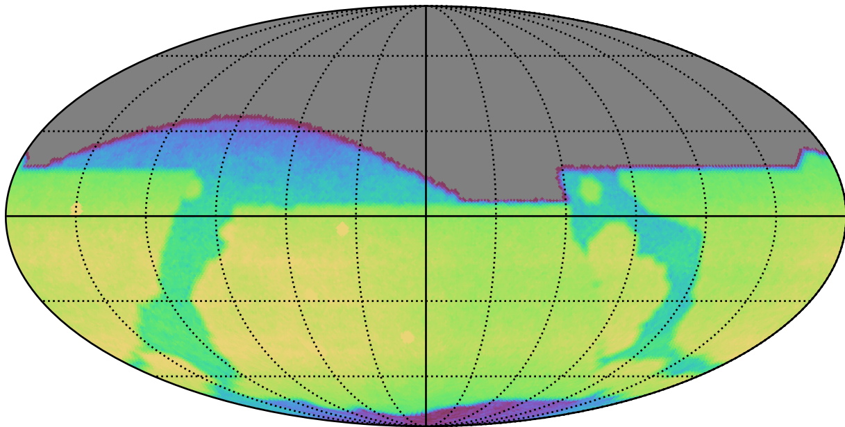
ddf_loaded_fl4_v3.4_10yrs All sky r band: CoaddM5
