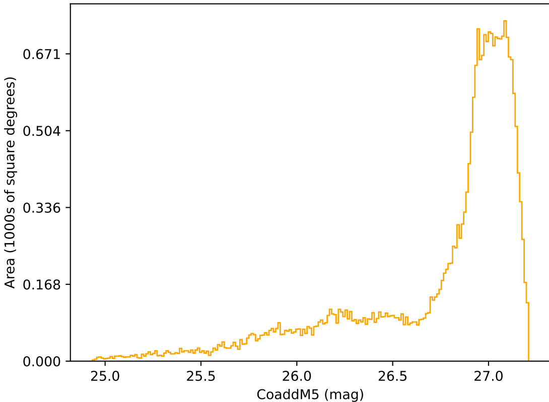
ddf_loaded_fl4_v3.4_10yrs All sky r band: CoaddM5
