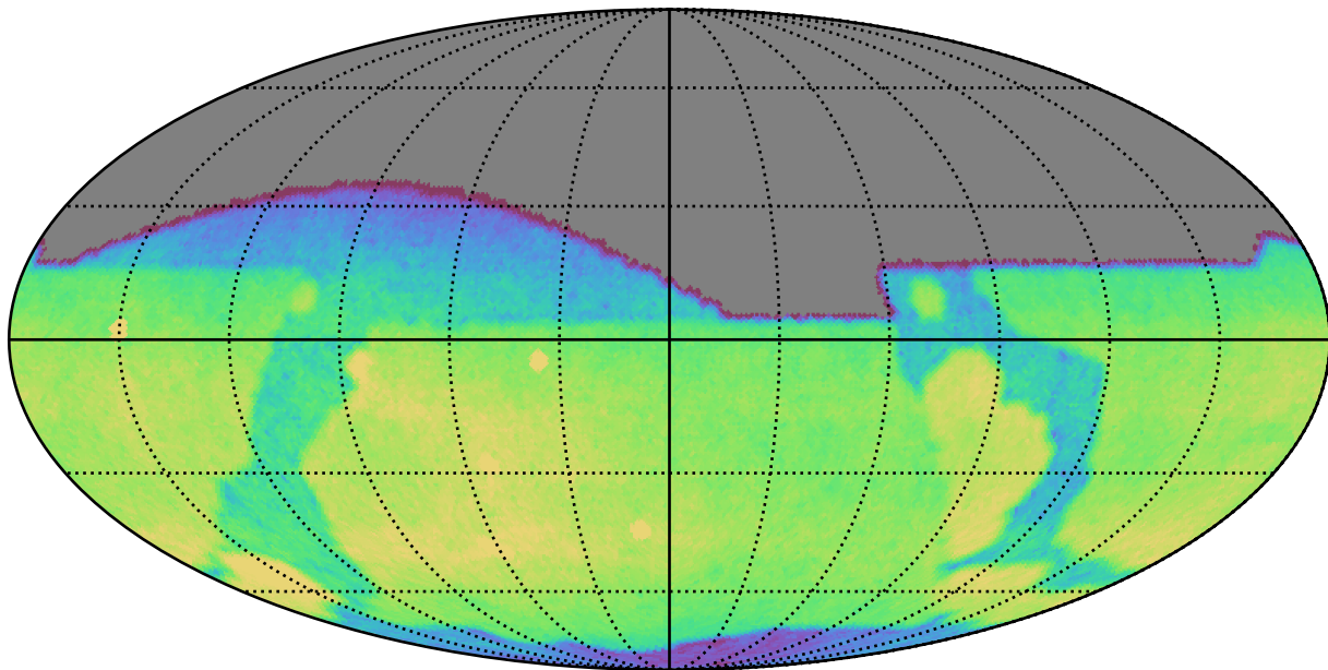
ddf_loaded_fl4_v3.4_10yrs All sky g band: CoaddM5
