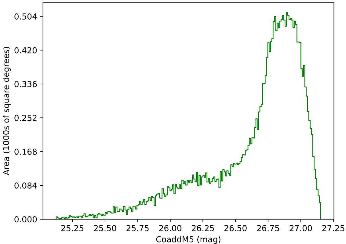
ddf_loaded_fl4_v3.4_10yrs All sky g band: CoaddM5
