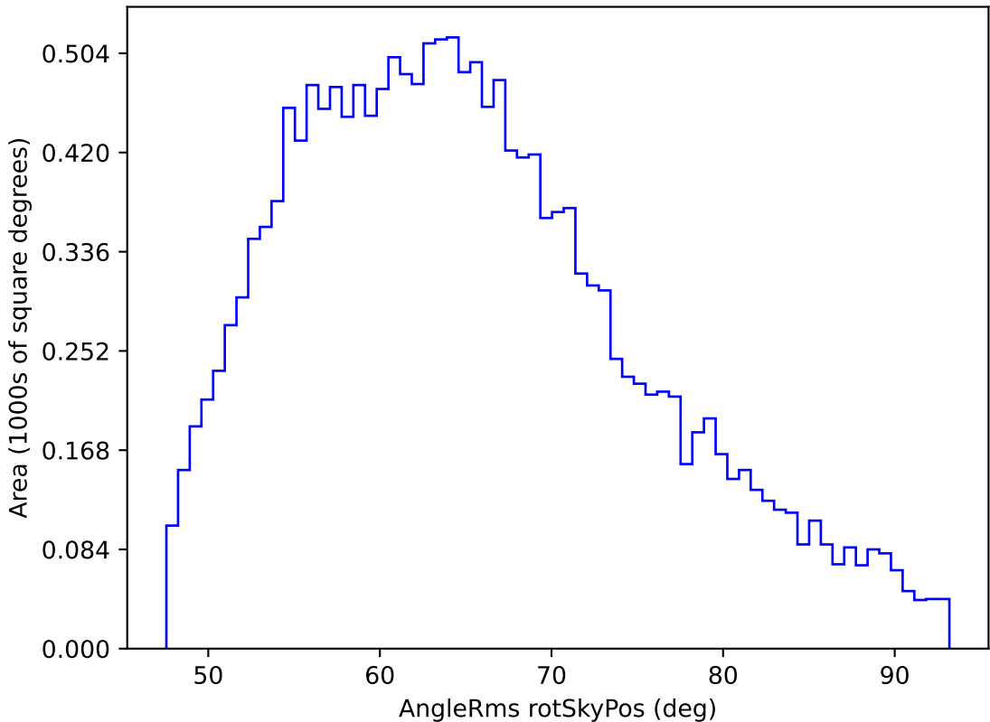
ddf_loaded_fl4_v3.4_10yrs WFD z band: AngleRms rotSkyPos
