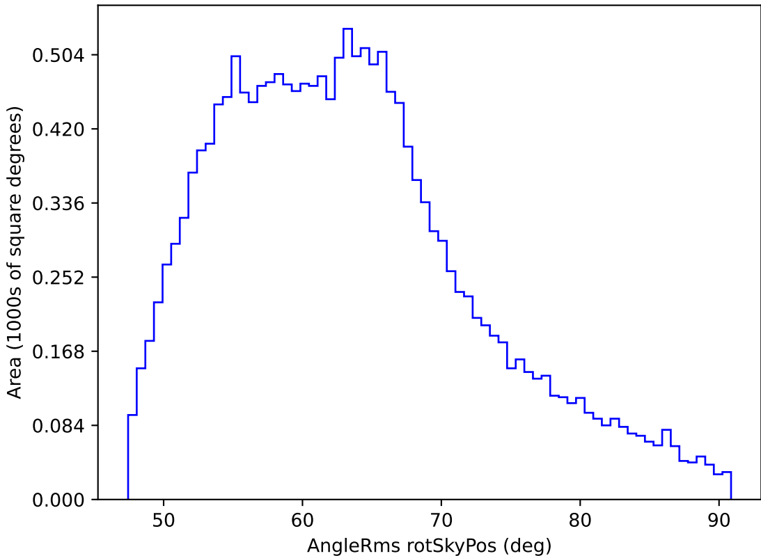
ddf_loaded_fl4_v3.4_10yrs WFD y band: AngleRms rotSkyPos
