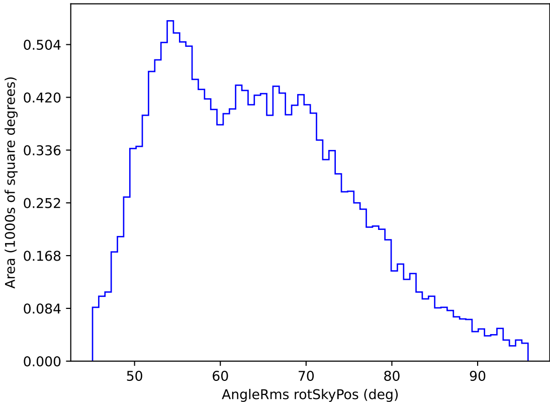
ddf_loaded_fl4_v3.4_10yrs WFD u band: AngleRms rotSkyPos
