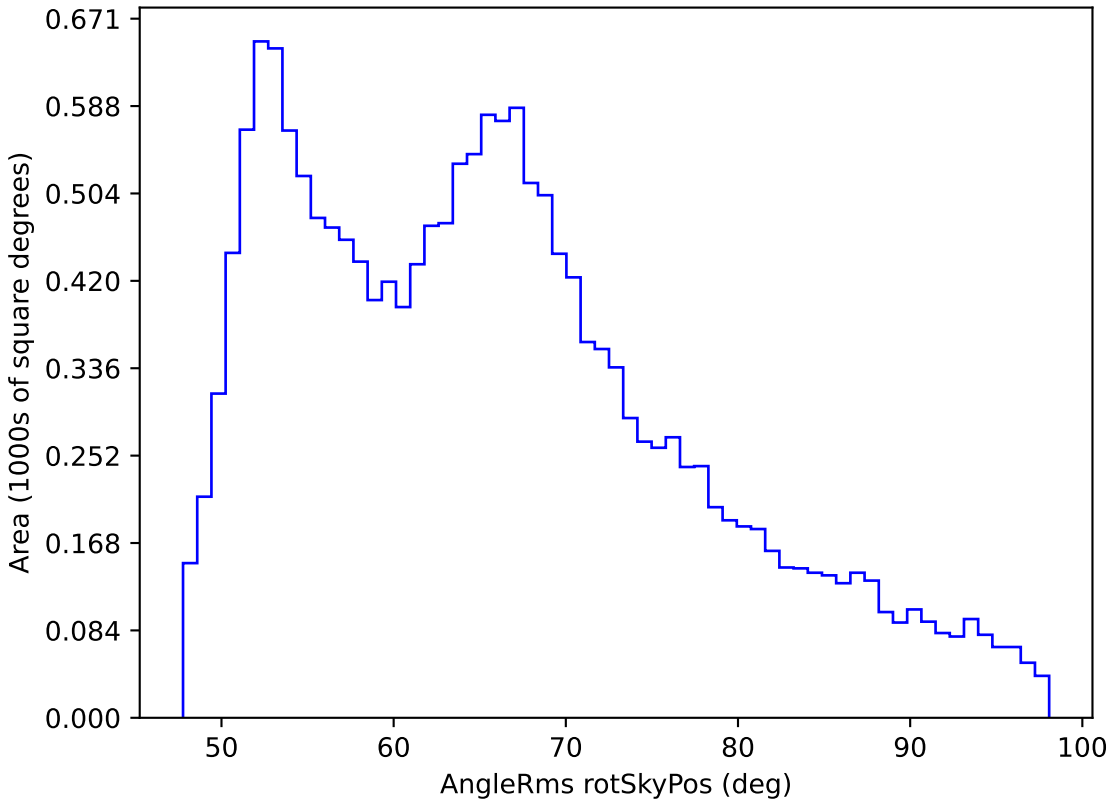
ddf_loaded_fl4_v3.4_10yrs WFD r band: AngleRms rotSkyPos
