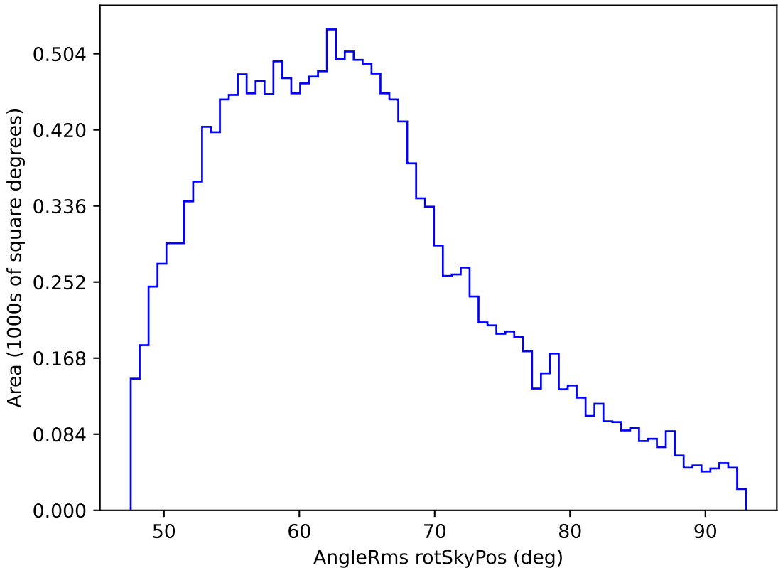
ddf_loaded_fl4_v3.4_10yrs WFD i band: AngleRms rotSkyPos
