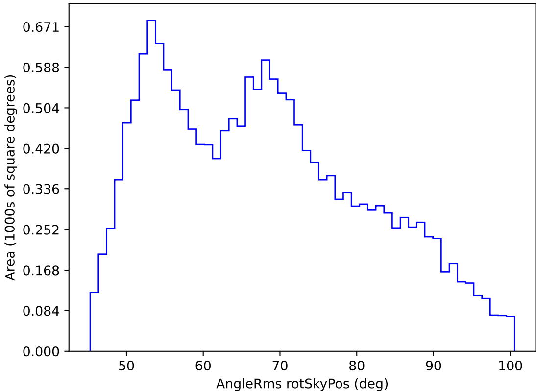
ddf_loaded_fl4_v3.4_10yrs WFD g band: AngleRms rotSkyPos
