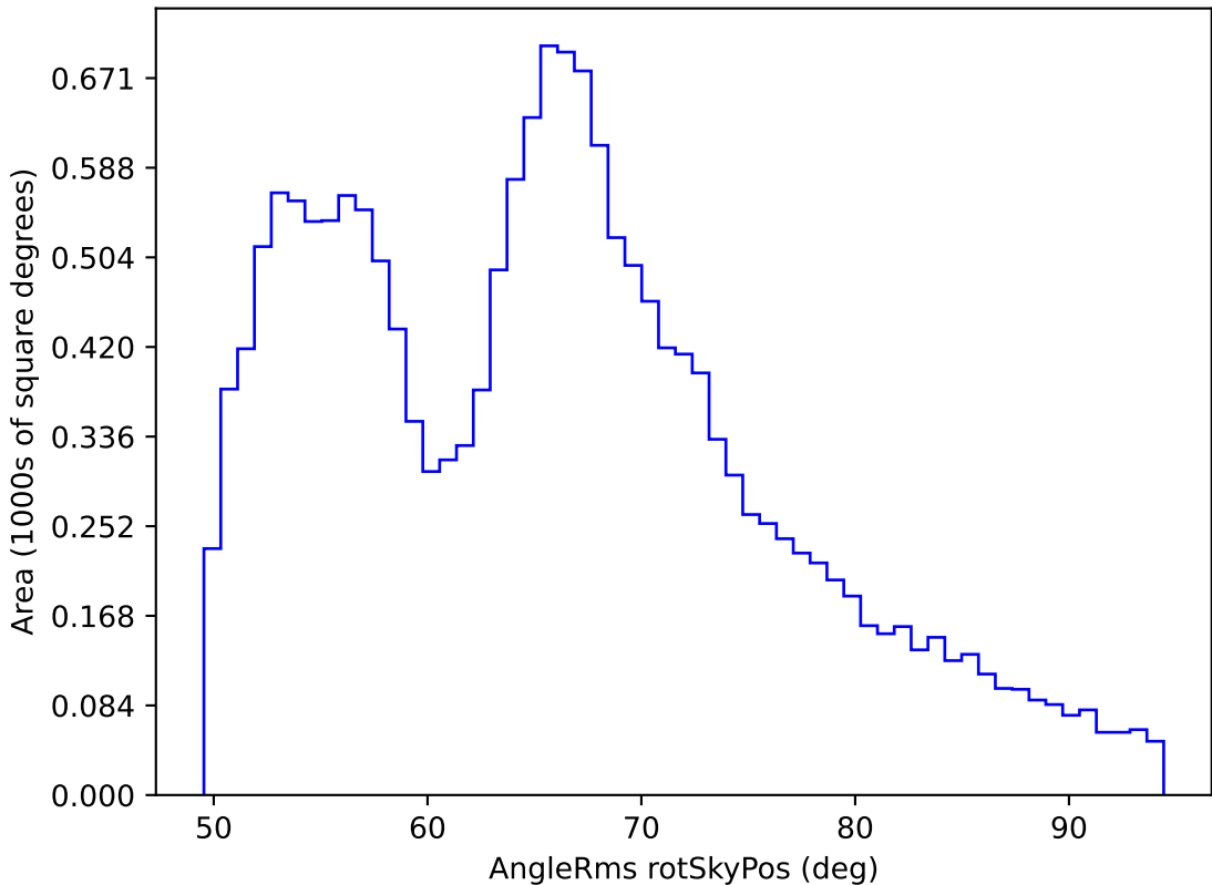
ddf_loaded_fl4_v3.4_10yrs WFD all bands: AngleRms rotSkyPos
