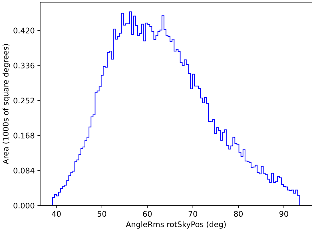
ddf_loaded_fl4_v3.4_10yrs All sky z band: AngleRms rotSkyPos
