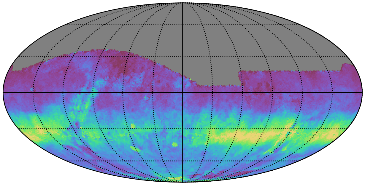
ddf_loaded_fl4_v3.4_10yrs All sky r band: AngleRms rotSkyPos
