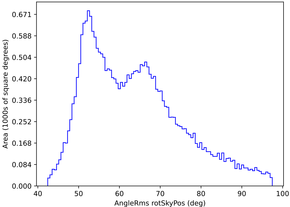
ddf_loaded_fl4_v3.4_10yrs All sky r band: AngleRms rotSkyPos
