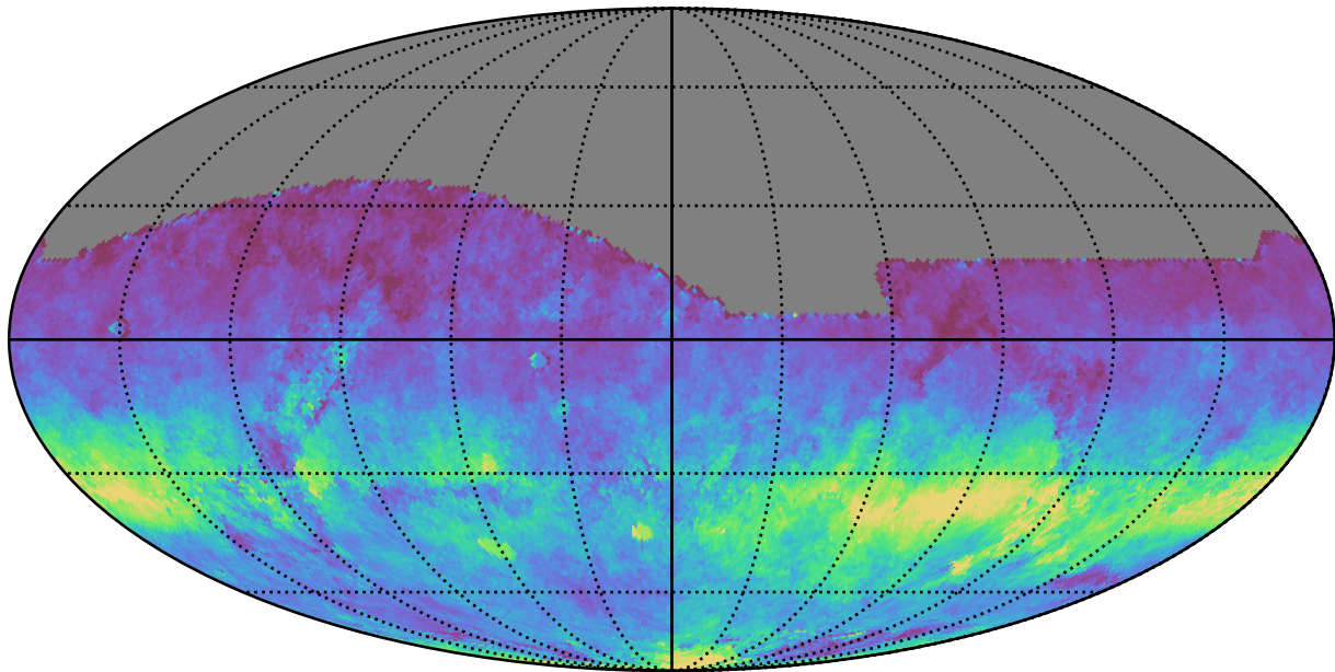
ddf_loaded_fl4_v3.4_10yrs All sky i band: AngleRms rotSkyPos
