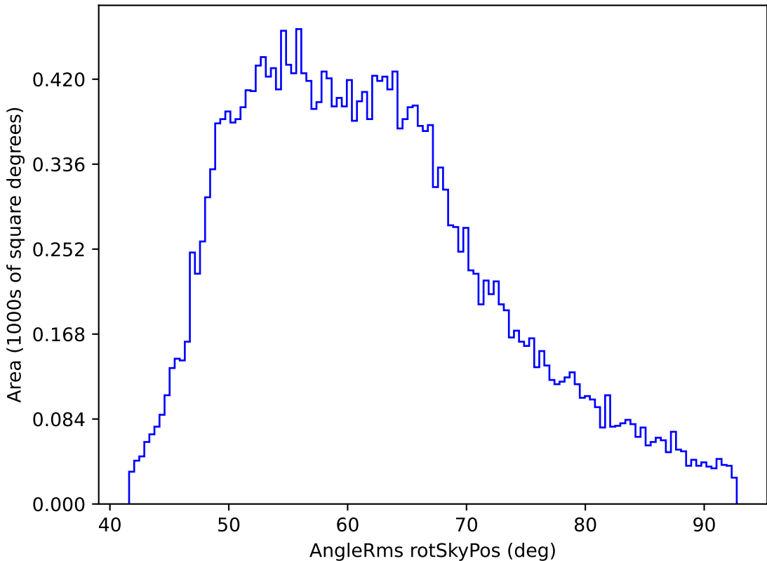
ddf_loaded_fl4_v3.4_10yrs All sky i band: AngleRms rotSkyPos
