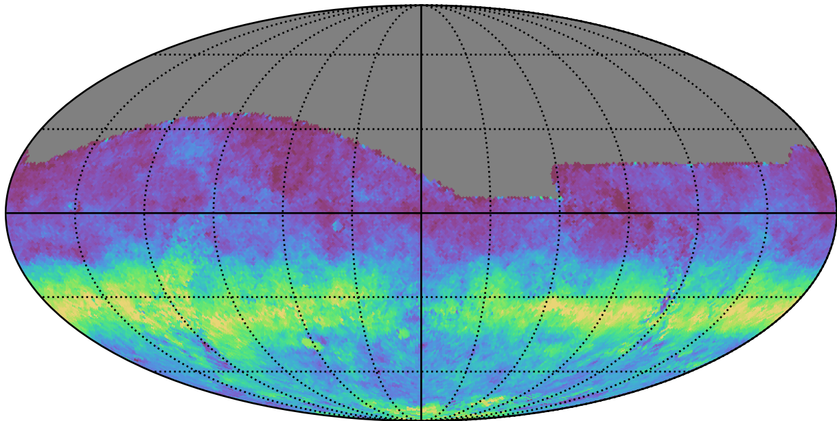
ddf_loaded_fl4_v3.4_10yrs All sky g band: AngleRms rotSkyPos
