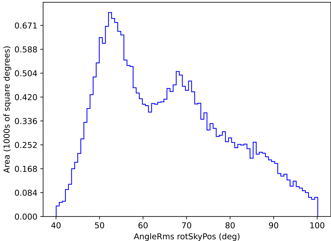
ddf_loaded_fl4_v3.4_10yrs All sky g band: AngleRms rotSkyPos
