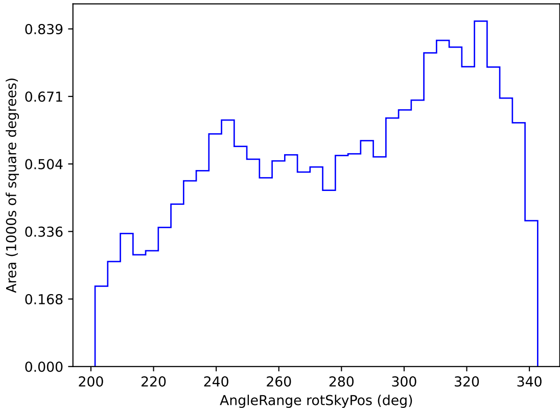
ddf_loaded_fl4_v3.4_10yrs WFD z band: AngleRange rotSkyPos
