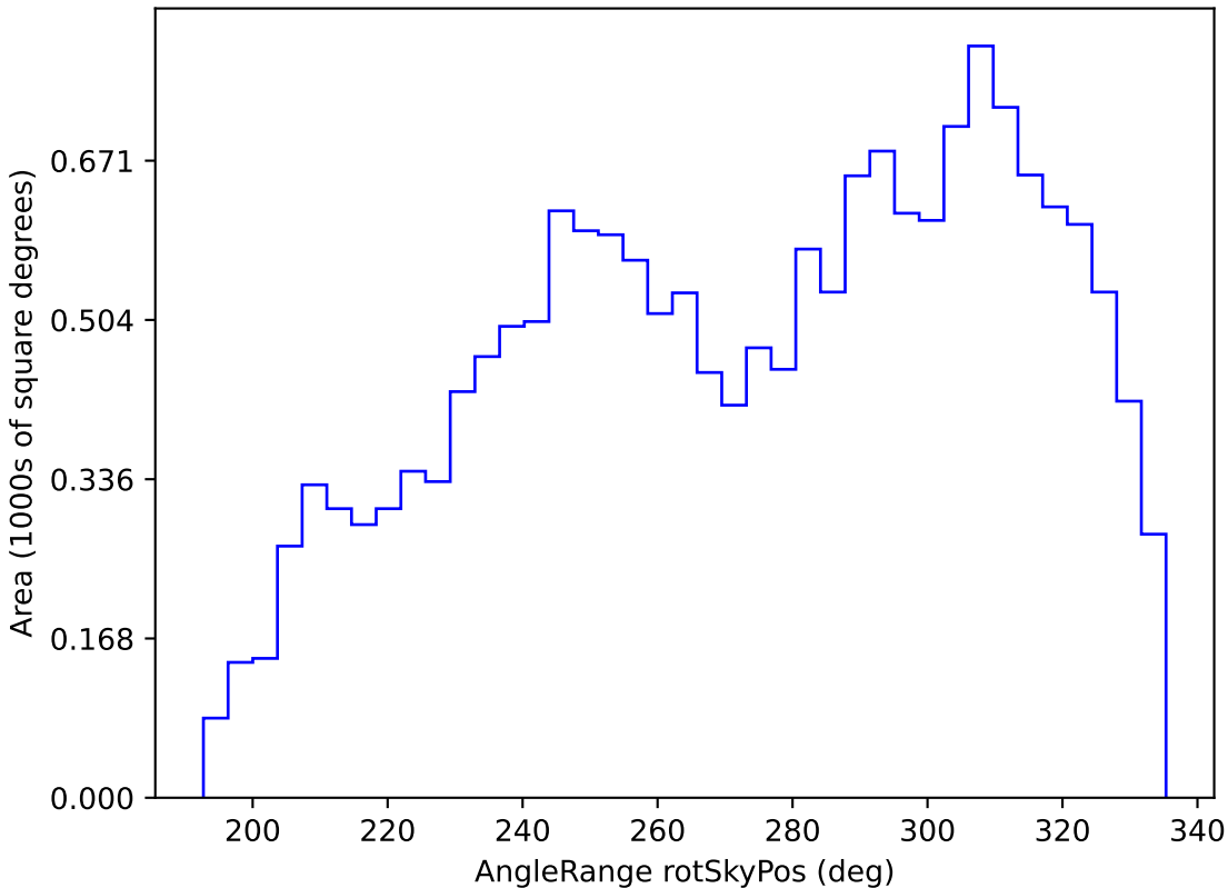
ddf_loaded_fl4_v3.4_10yrs WFD y band: AngleRange rotSkyPos
