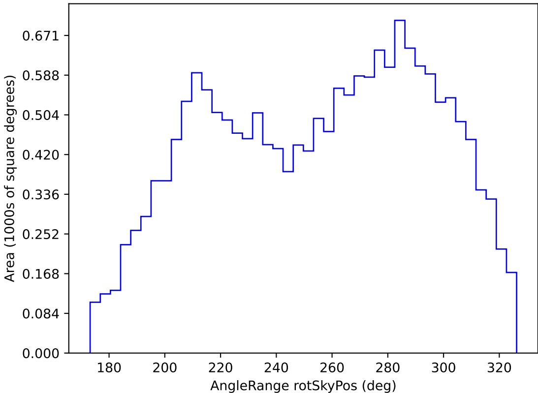
ddf_loaded_fl4_v3.4_10yrs WFD u band: AngleRange rotSkyPos
