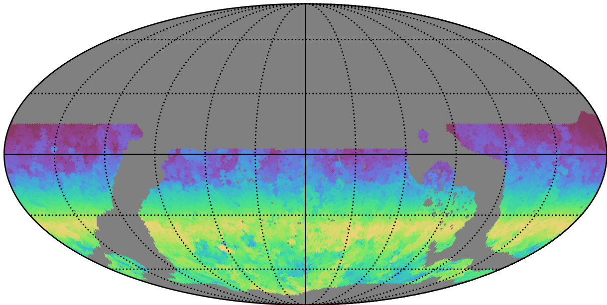
ddf_loaded_fl4_v3.4_10yrs WFD r band: AngleRange rotSkyPos
