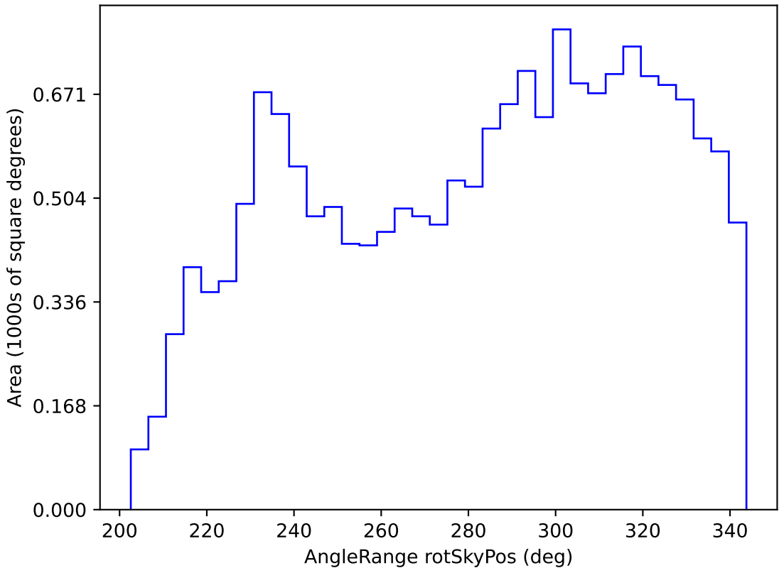
ddf_loaded_fl4_v3.4_10yrs WFD r band: AngleRange rotSkyPos
