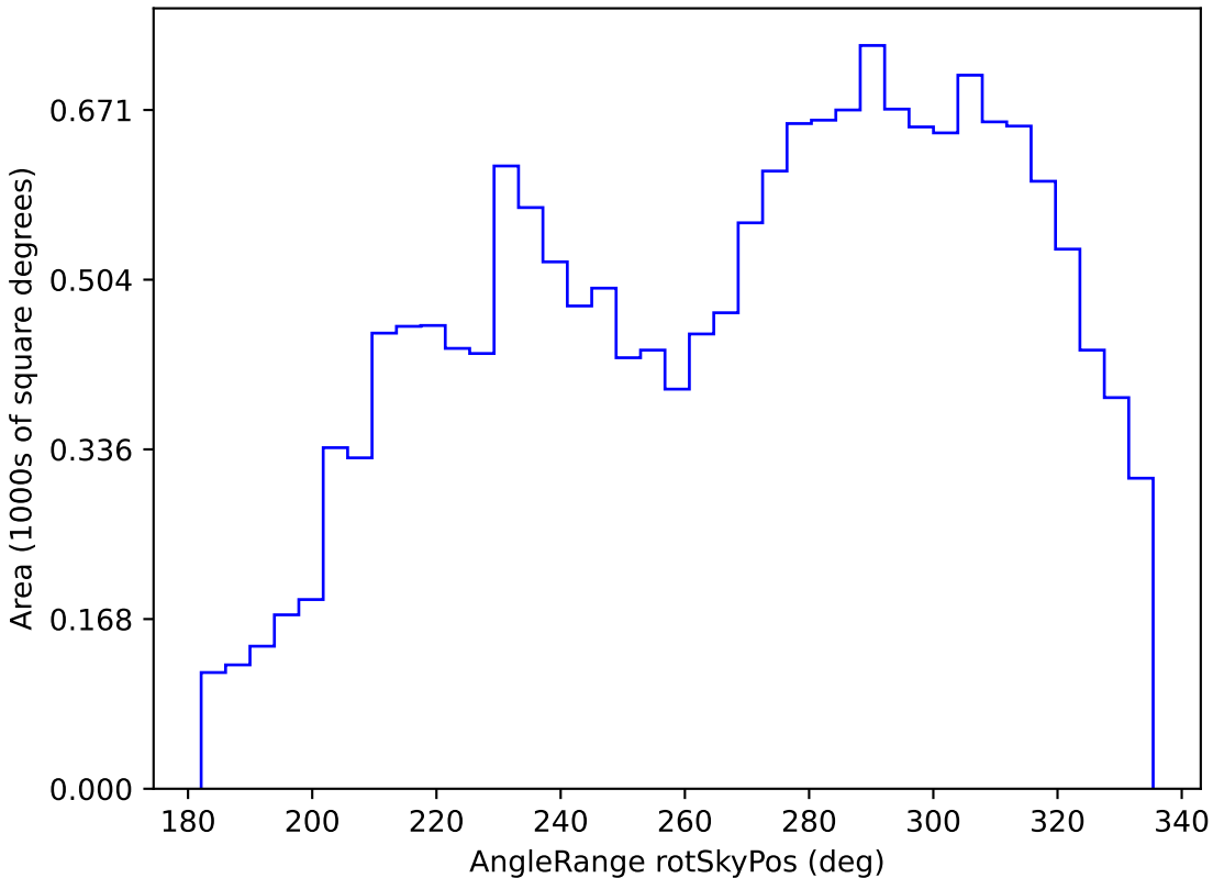
ddf_loaded_fl4_v3.4_10yrs WFD g band: AngleRange rotSkyPos
