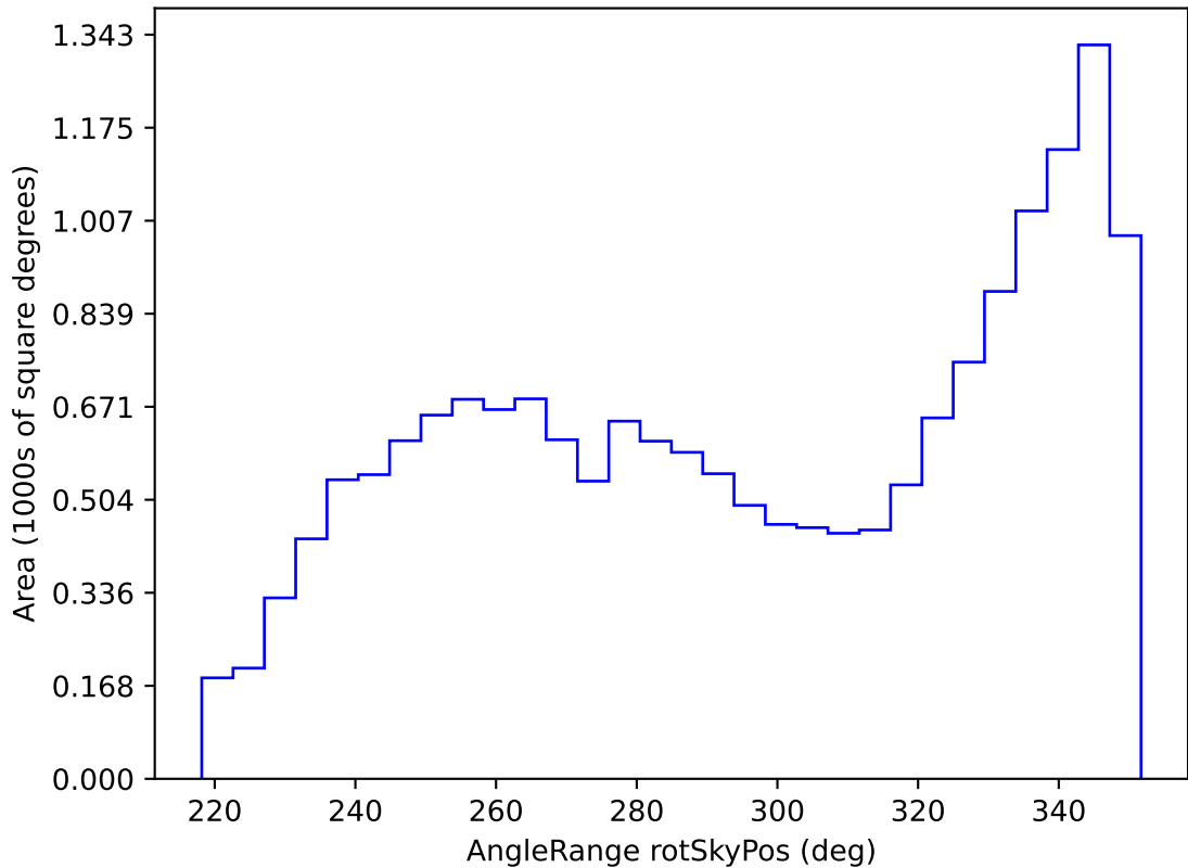
ddf_loaded_fl4_v3.4_10yrs WFD all bands: AngleRange rotSkyPos
