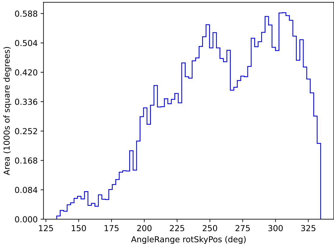
ddf_loaded_fl4_v3.4_10yrs All sky y band: AngleRange rotSkyPos
