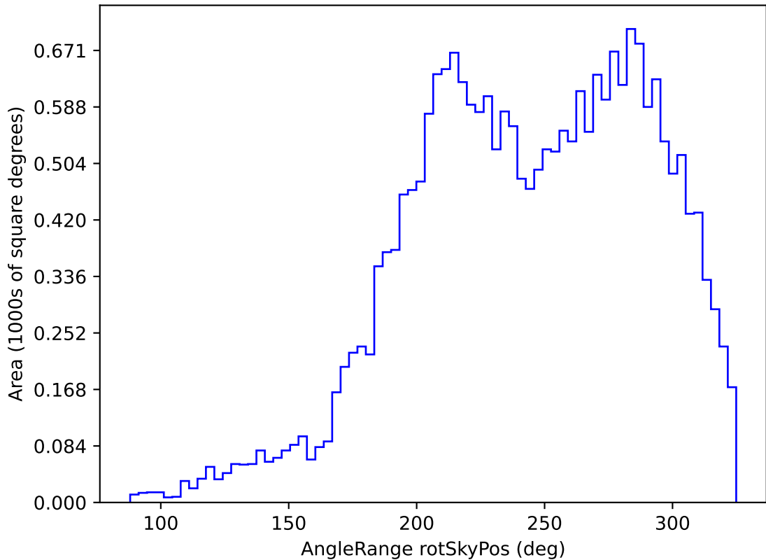
ddf_loaded_fl4_v3.4_10yrs All sky u band: AngleRange rotSkyPos
