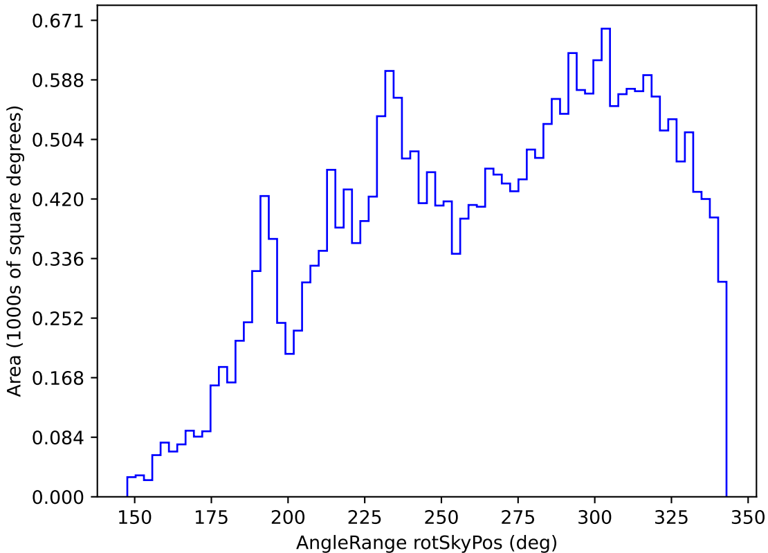
ddf_loaded_fl4_v3.4_10yrs All sky r band: AngleRange rotSkyPos
