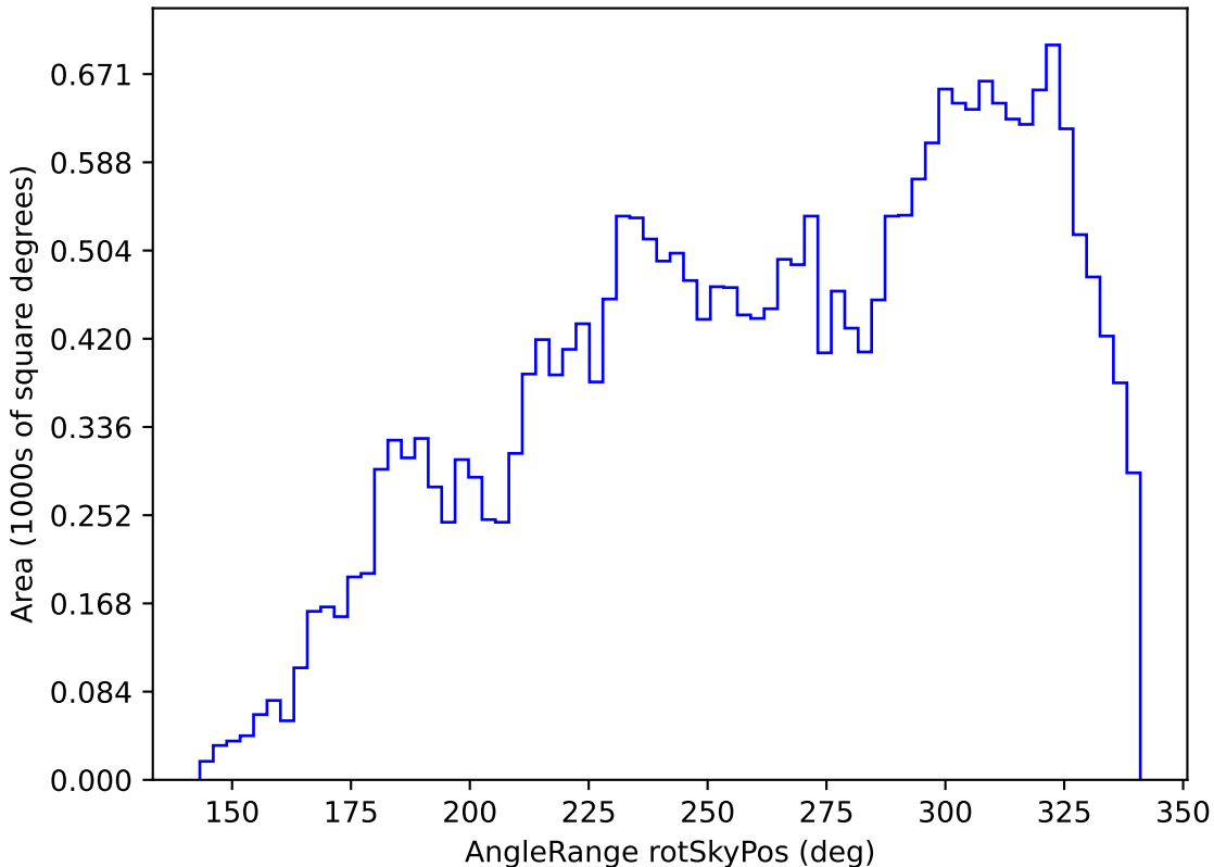
ddf_loaded_fl4_v3.4_10yrs All sky i band: AngleRange rotSkyPos
