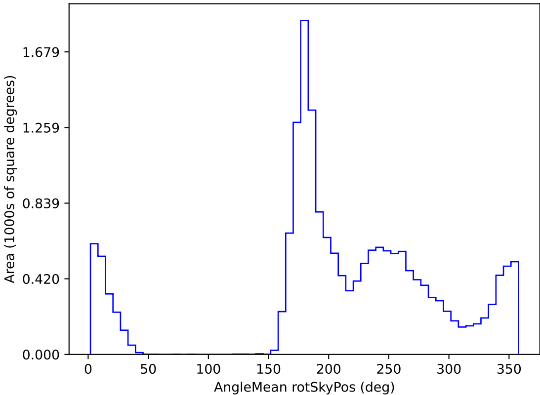
ddf_loaded_fl4_v3.4_10yrs WFD z band: AngleMean rotSkyPos
