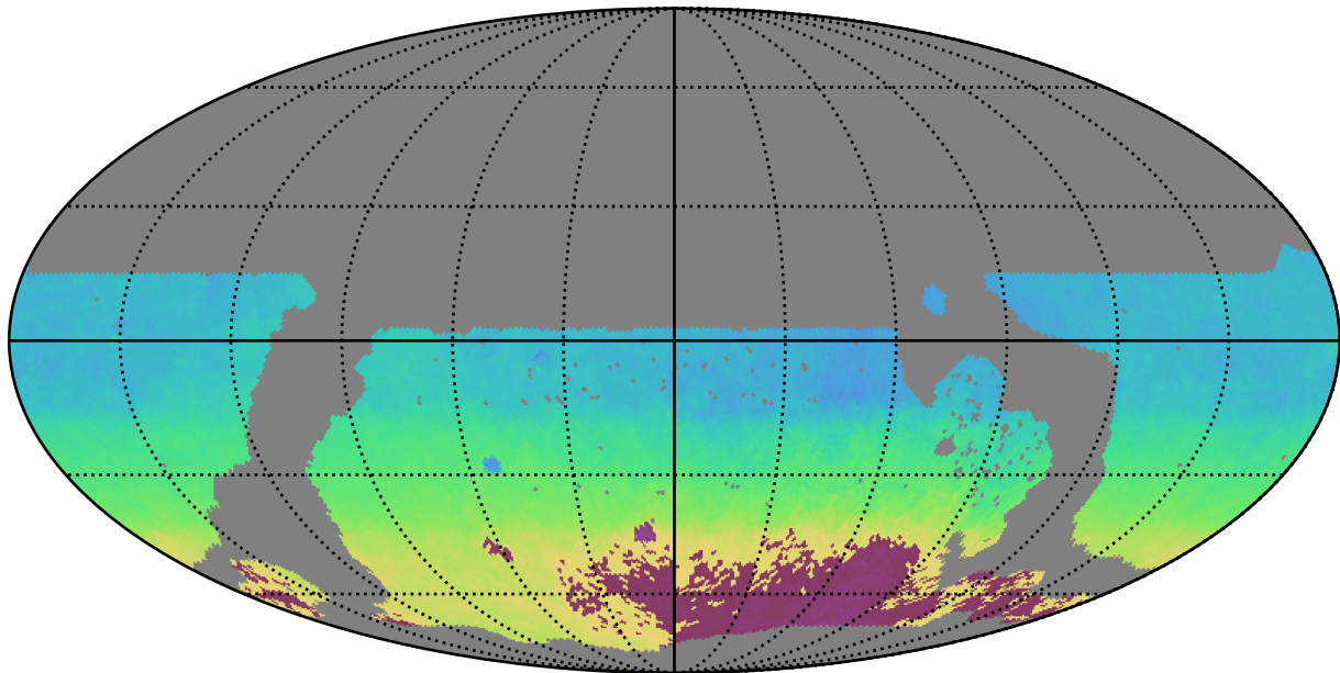
ddf_loaded_fl4_v3.4_10yrs WFD y band: AngleMean rotSkyPos
