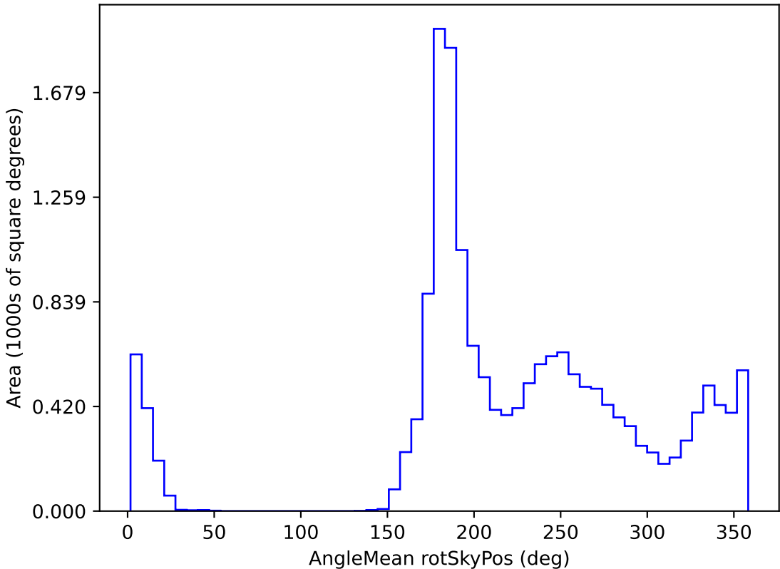
ddf_loaded_fl4_v3.4_10yrs WFD y band: AngleMean rotSkyPos
