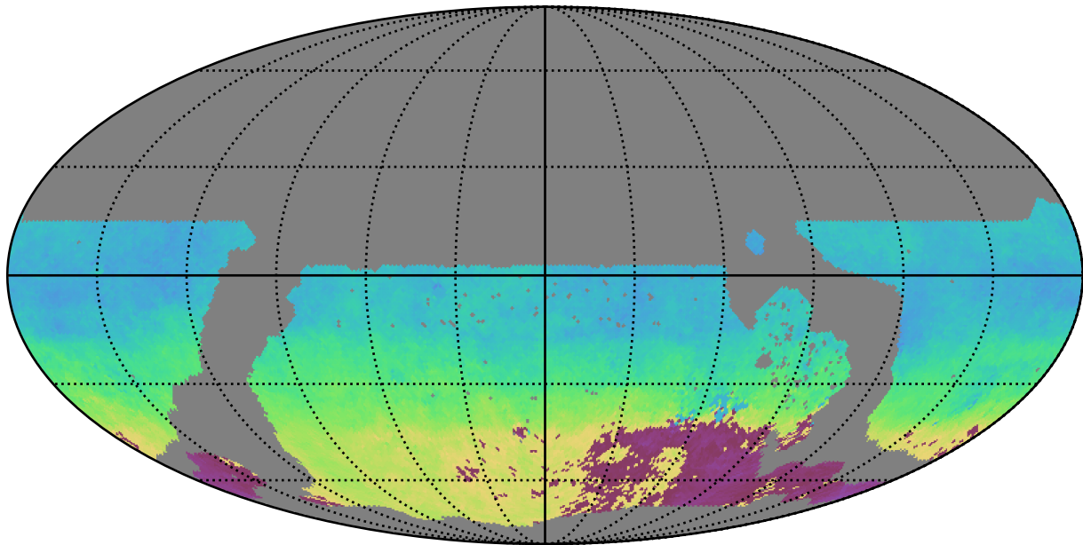
ddf_loaded_fl4_v3.4_10yrs WFD u band: AngleMean rotSkyPos
