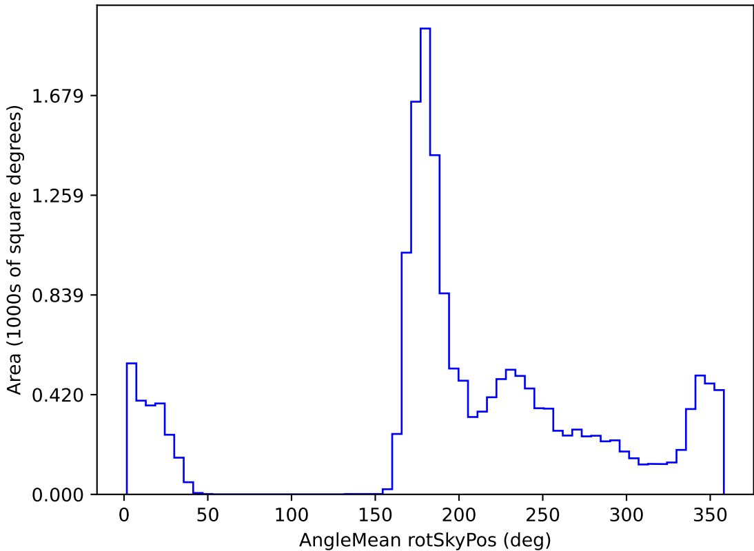
ddf_loaded_fl4_v3.4_10yrs WFD r band: AngleMean rotSkyPos
