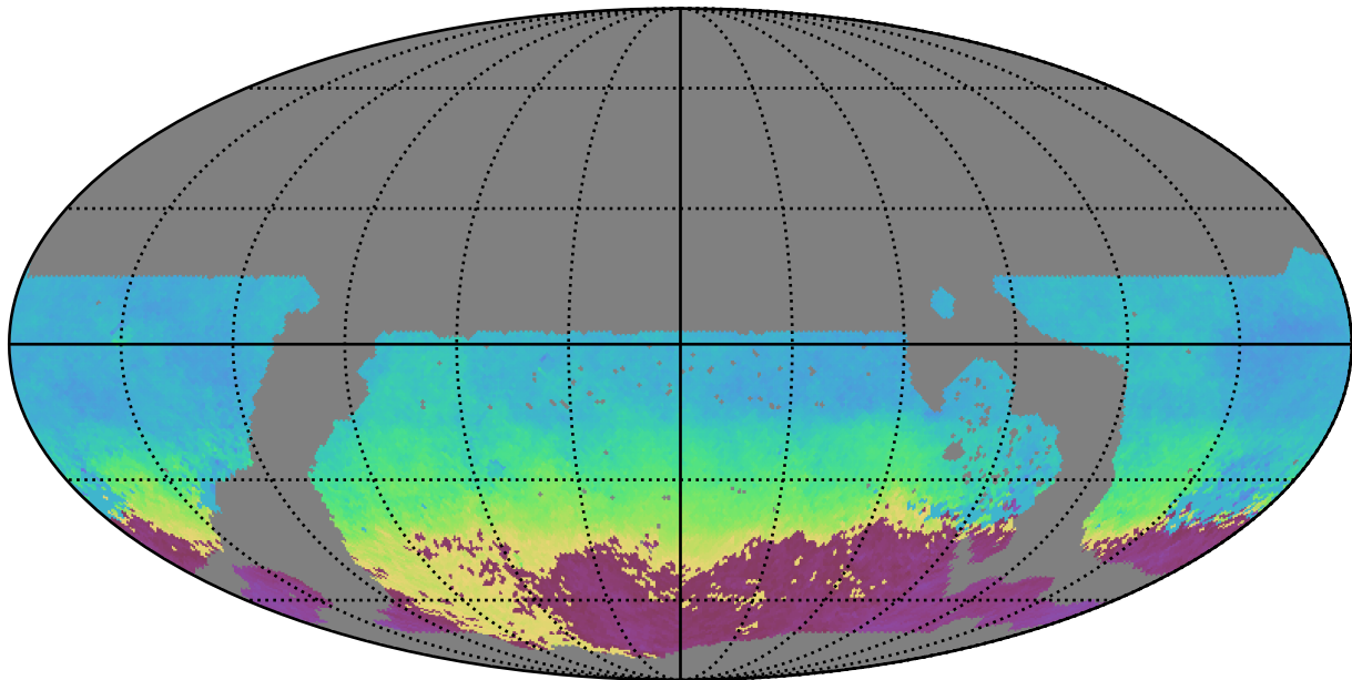
ddf_loaded_fl4_v3.4_10yrs WFD g band: AngleMean rotSkyPos
