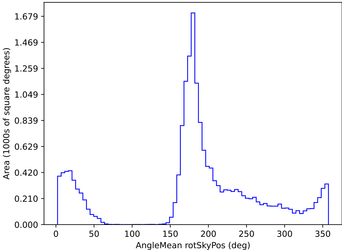
ddf_loaded_fl4_v3.4_10yrs WFD g band: AngleMean rotSkyPos
