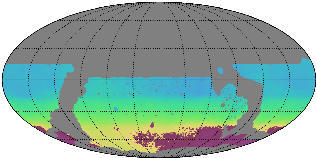
ddf_loaded_fl4_v3.4_10yrs WFD all bands: AngleMean rotSkyPos
