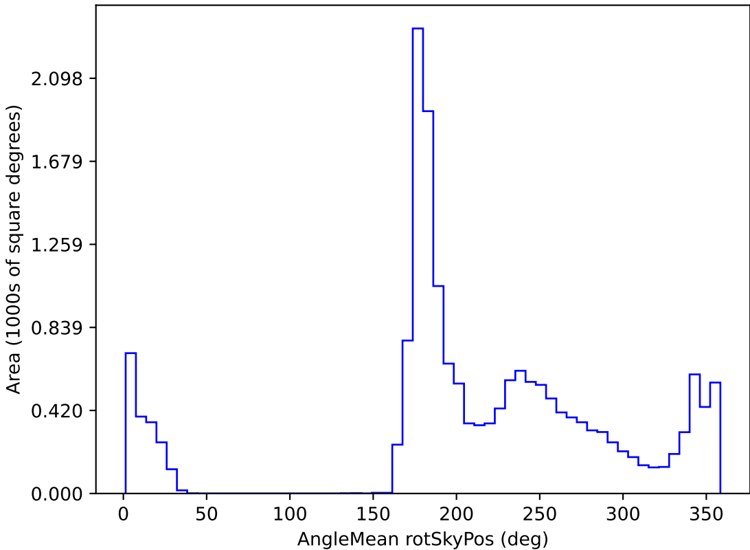
ddf_loaded_fl4_v3.4_10yrs WFD all bands: AngleMean rotSkyPos
