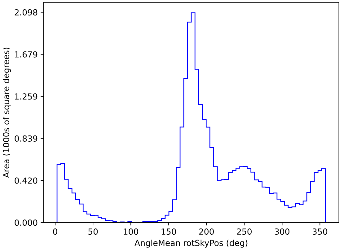
ddf_loaded_fl4_v3.4_10yrs All sky z band: AngleMean rotSkyPos
