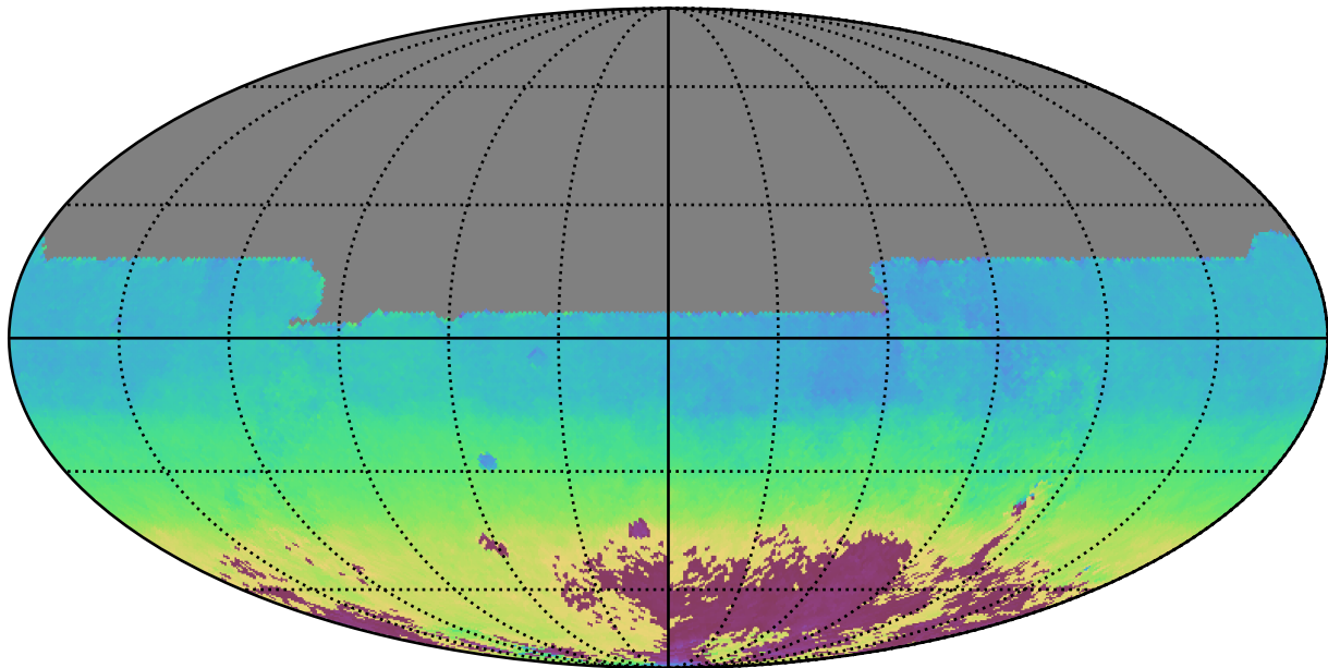
ddf_loaded_fl4_v3.4_10yrs All sky y band: AngleMean rotSkyPos
