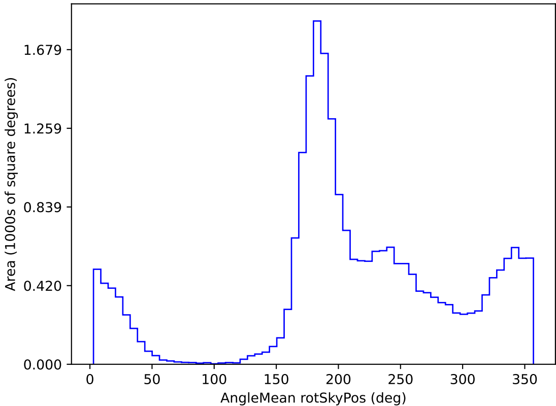
ddf_loaded_fl4_v3.4_10yrs All sky u band: AngleMean rotSkyPos
