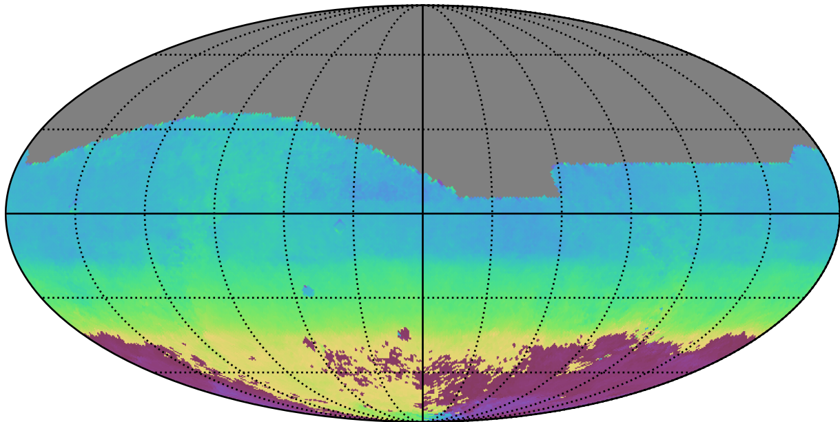
ddf_loaded_fl4_v3.4_10yrs All sky i band: AngleMean rotSkyPos
