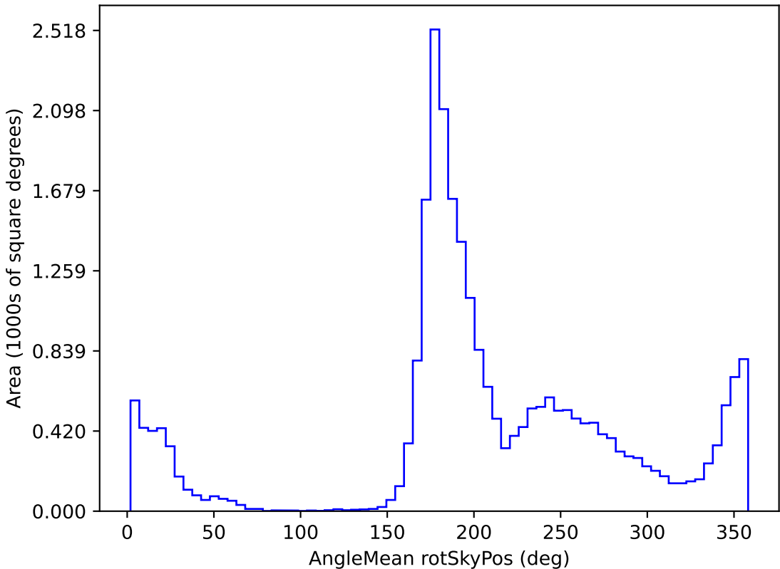
ddf_loaded_fl4_v3.4_10yrs All sky i band: AngleMean rotSkyPos
