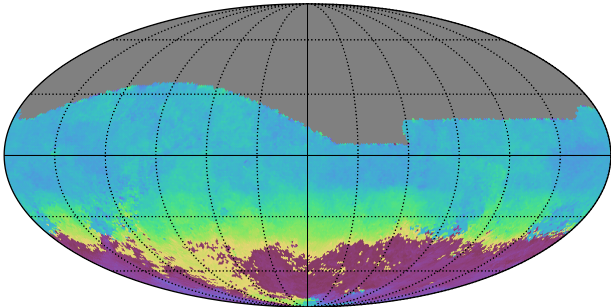
ddf_loaded_fl4_v3.4_10yrs All sky g band: AngleMean rotSkyPos
