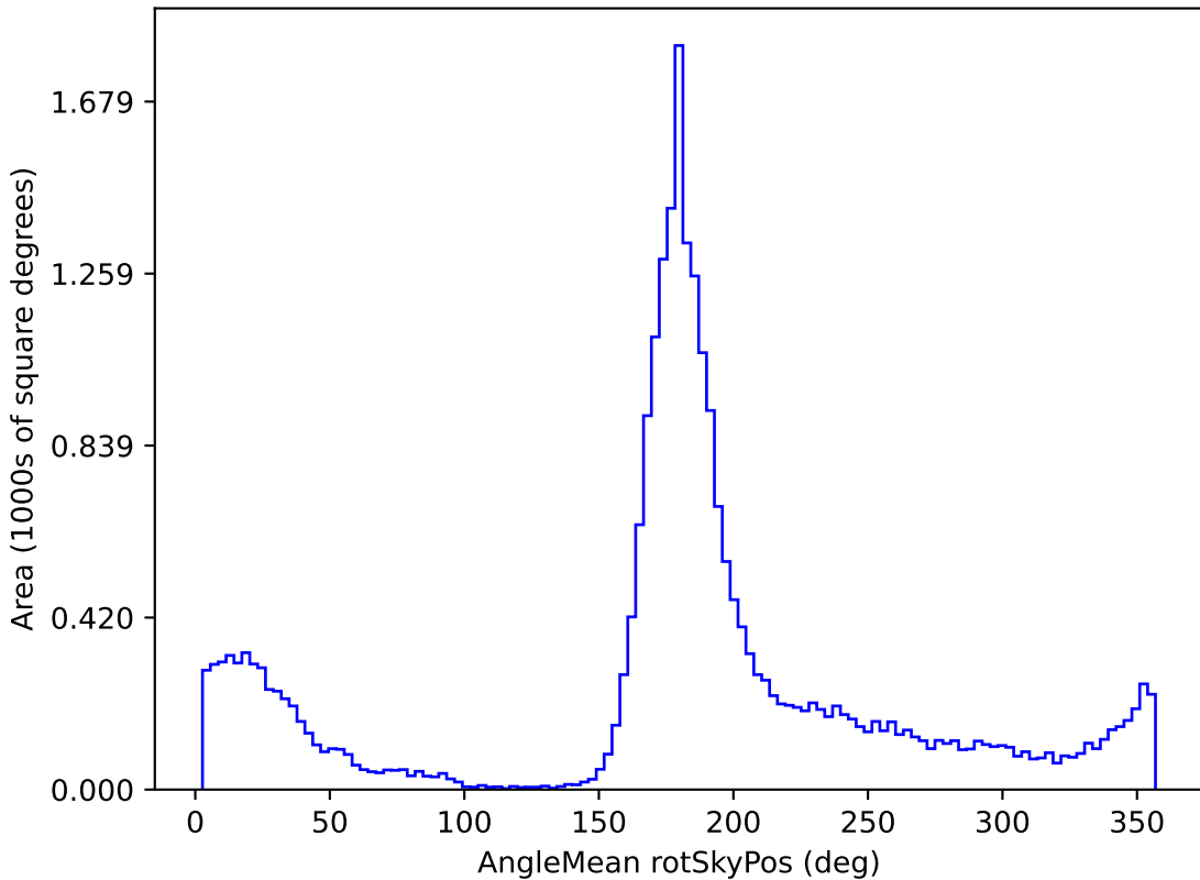
ddf_loaded_fl4_v3.4_10yrs All sky g band: AngleMean rotSkyPos
