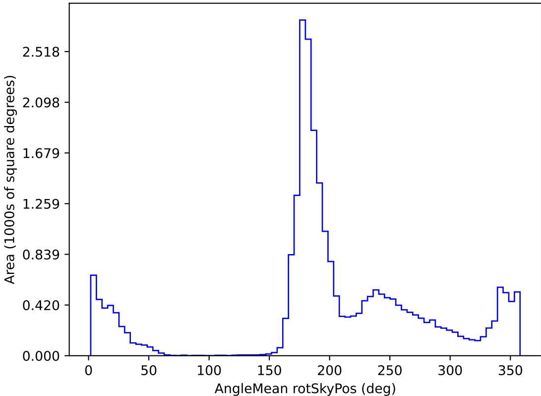
ddf_loaded_fl4_v3.4_10yrs All sky all bands: AngleMean rotSkyPos
