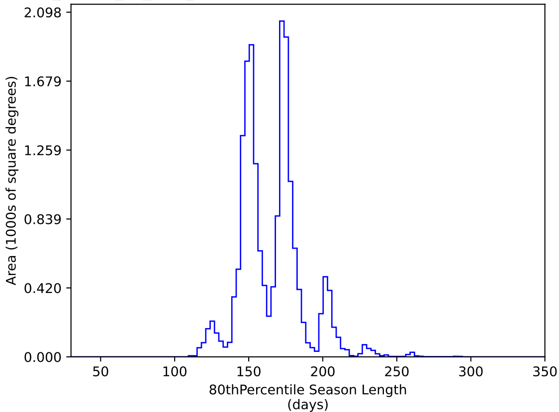
ddf_loaded_fl4_v3.4_10yrs WFD y band: 80thPercentile Season Length
