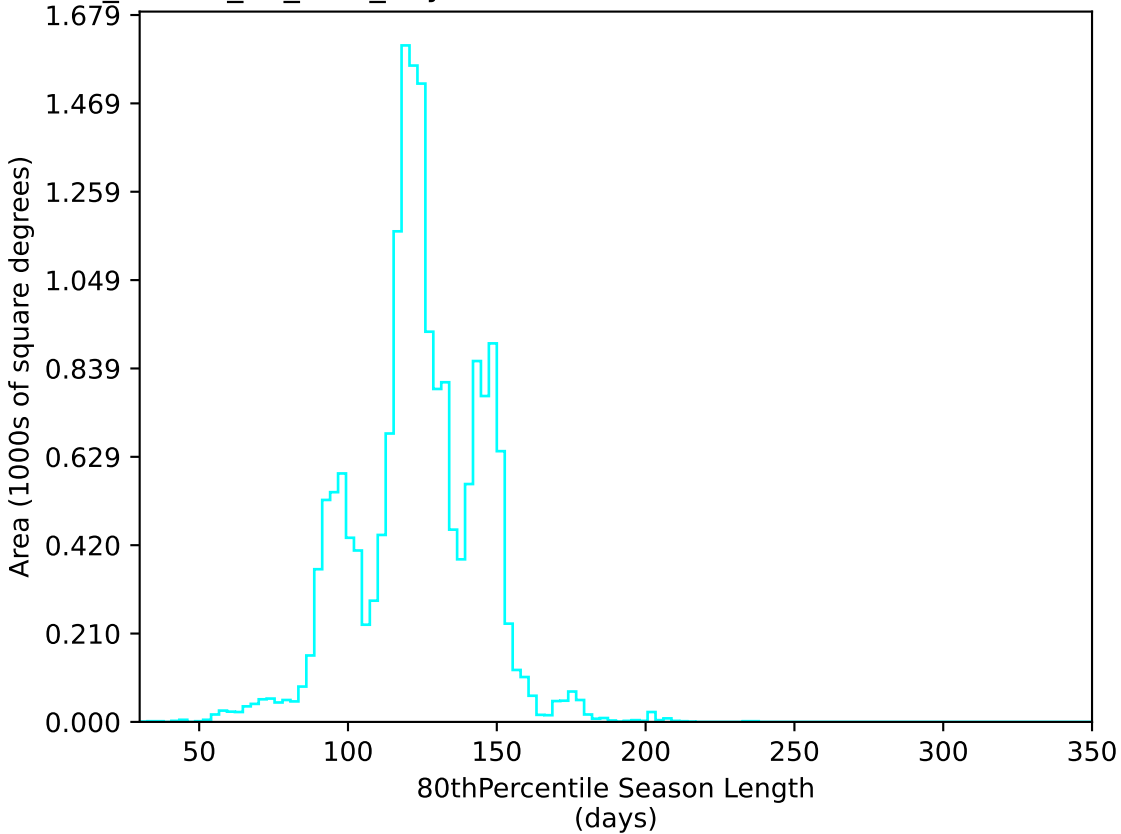
ddf_loaded_fl4_v3.4_10yrs WFD u band: 80thPercentile Season Length
