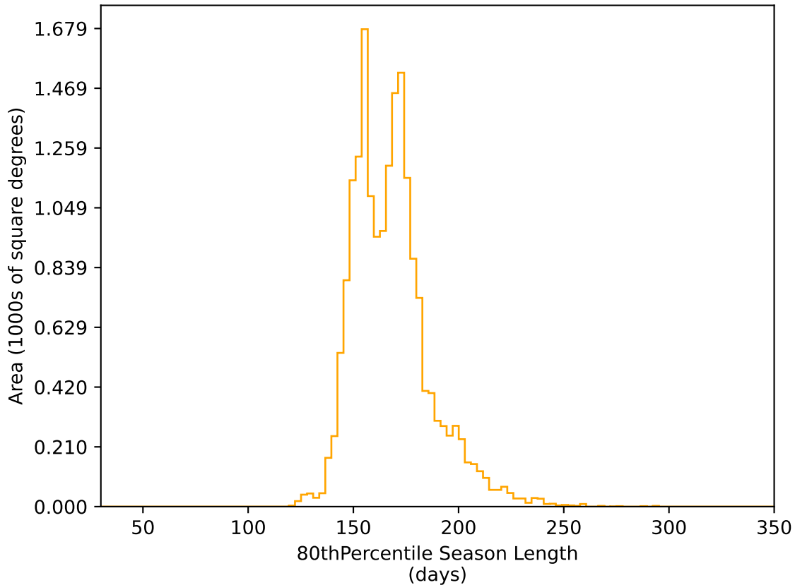
ddf_loaded_fl4_v3.4_10yrs WFD r band: 80thPercentile Season Length
