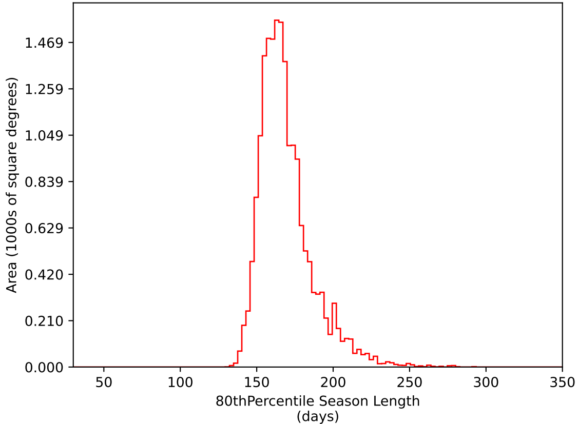
ddf_loaded_fl4_v3.4_10yrs WFD i band: 80thPercentile Season Length
